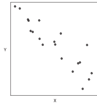
Correlation coefficient ( r = -0.9 ). Negative linear relationship.
